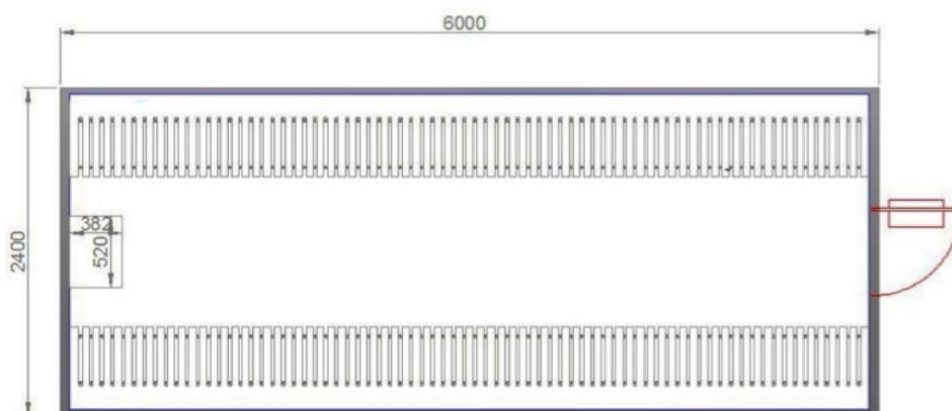
SECTION ISO 20' ARMORY
