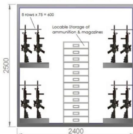
SECTION ISO 20' ARMORY
